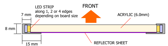
Heat Sink Option 'Type B' (7mm to front - 15mm to reverse)
